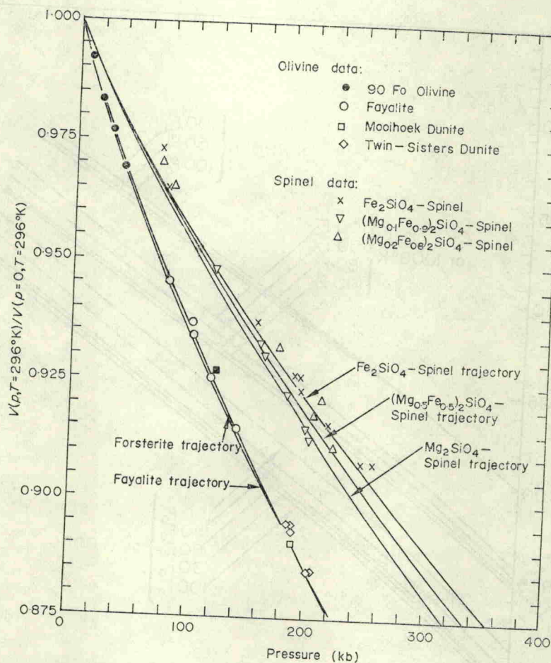
FIG. 8. Comparison of the calculated pressure-volume relation of olivine with experimental compression data. The solid lines are the present work, independent of compression data points. The isothermal compression data of olivine are due to Bridgman (●) and to Takahashi (○). The shock compression data are due to McQueen, Marsh, & Fritz for Mooihoek dunite (□) and Twin-Sisters dunite (◇). The isothermal compression data of olivine-transformed spinels are due to Mao et al. (1969), and the solid lines are the calculated pressure-volume relation for the olivine-transformed spinels in the \text{Mg}_2\text{SiO}_4 - \text{Fe}_2\text{SiO}_4 series established by Chung (1971b).
